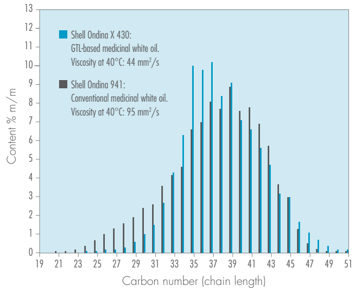
Figure 2: The carbon number distribution of Shell Ondina X 430 is comparable to that of a conventional medicinal white oil with a higher viscosity (Shell Ondina 941). Source: Shell.
