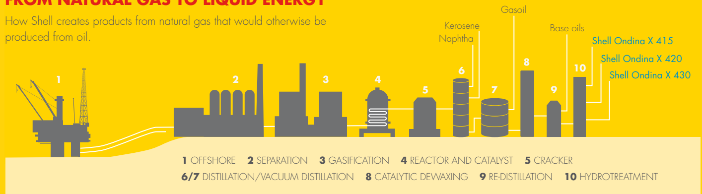
Figure 1: The GTL process converts clean-burning natural gas into cleaner-burning fuels and high-quality base oils through the Fischer-Tropsch process. GTL base oils are further processed to produce high-quality medicinal white oils. Source: Shell.
